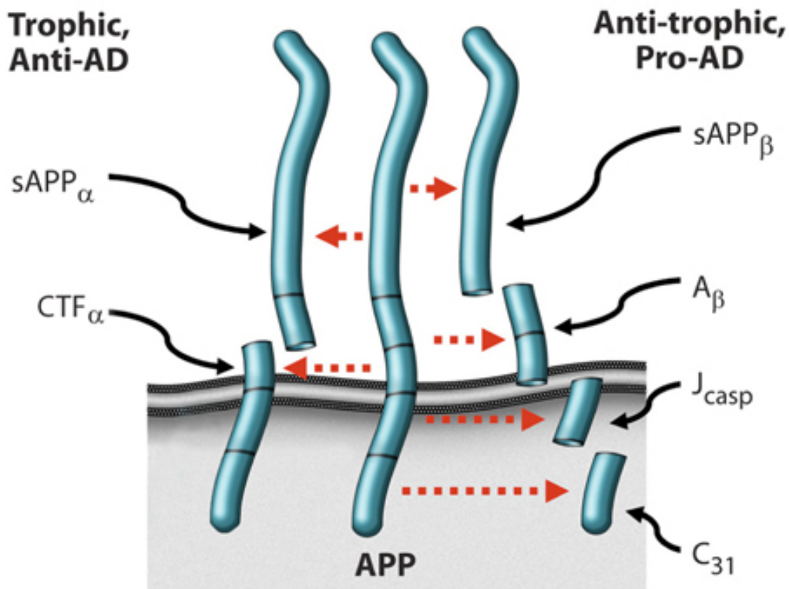
Figure 1. Alternative processing of, and signaling by, APP. [5].
